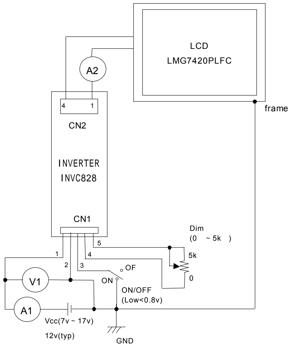
Fig.1 Wiring
