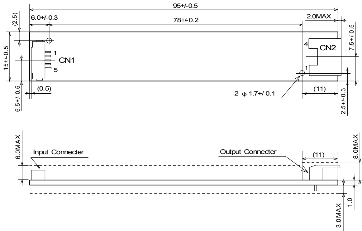
Fig.3 Dimensional Outline
